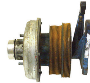
BorgWarner-, Kysor- and Kit Masters-style Fan Drives Complete with Drive Hub
