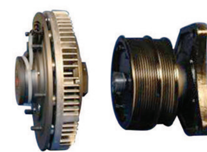
Concepts/LICOS Fan Drives Complete with Fan Drive Hub
